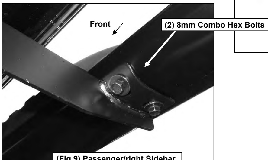
(Fig 9) Passenger/right Sidebar attached to Bracket pictured
