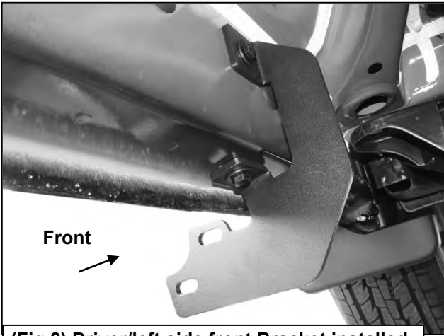
(Fig 8) Driver/left side front Bracket installed
