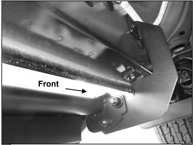
(Fig 12) Driver side front Complete install
