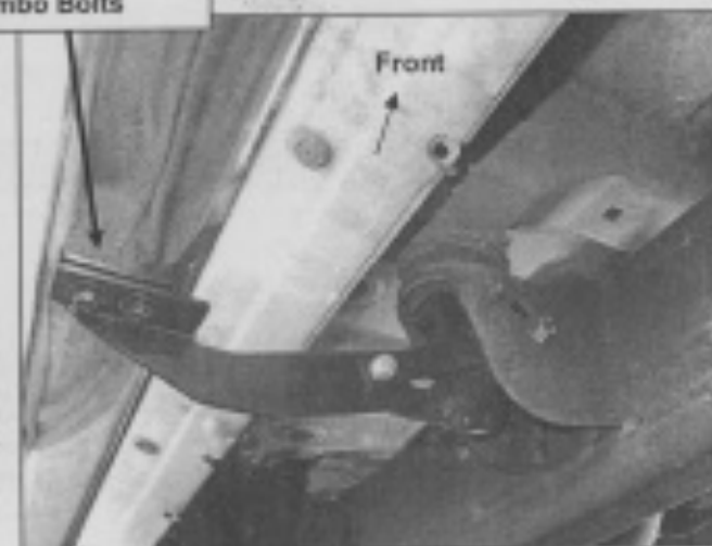
(Fig 13) Passenger side Center Bracket Installation
