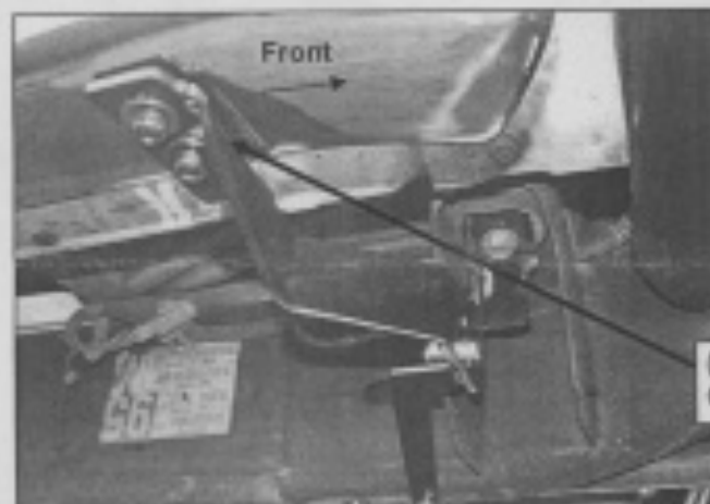
(Fig 12) Passenger side Front Bracket Installation
