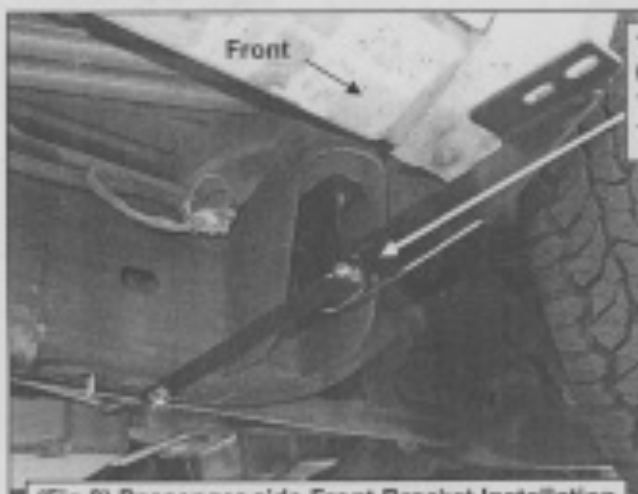
(Fig 8) Passenger side Front Bracket Installation
