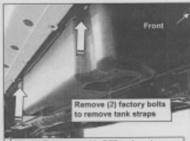
(Fig 11) Passenger side DEF tank and cover
