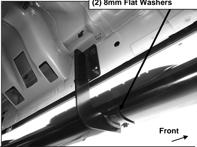
(Fig 5) Driver/left front Bracket installation pictured
