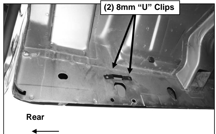
(Fig 6) Driver/left side rear mounting location
