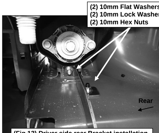
(Fig 13) Driver side rear Bracket installation
