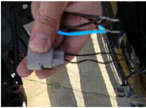
Step 15: splice the two ground wires from the housing to the black wires from the harness.
