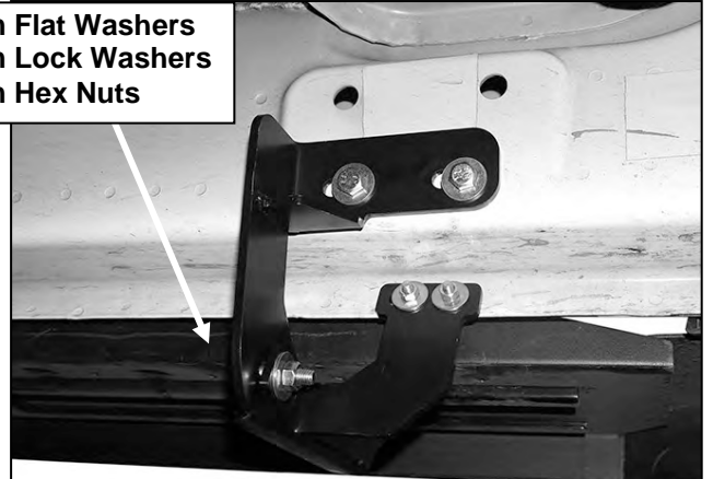
(Fig 17) Driver/left front Bracket assembly
