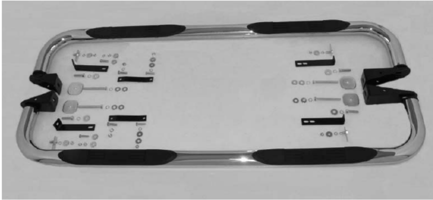
FULL ASSEMBLY -
