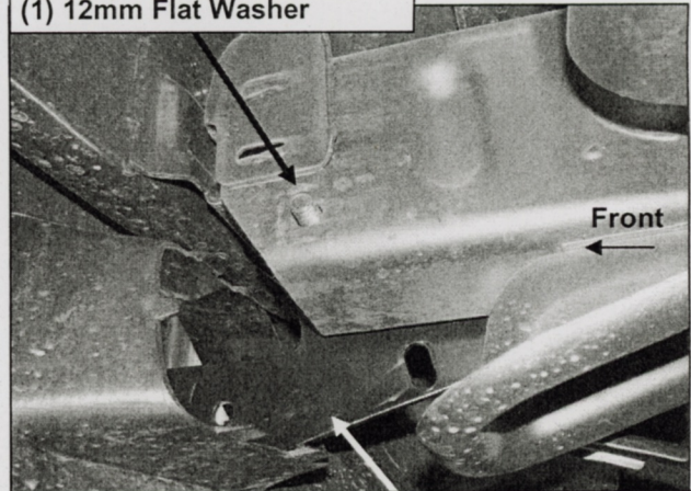
(Fig 4) Passenger side Mounting Bracket pictured
