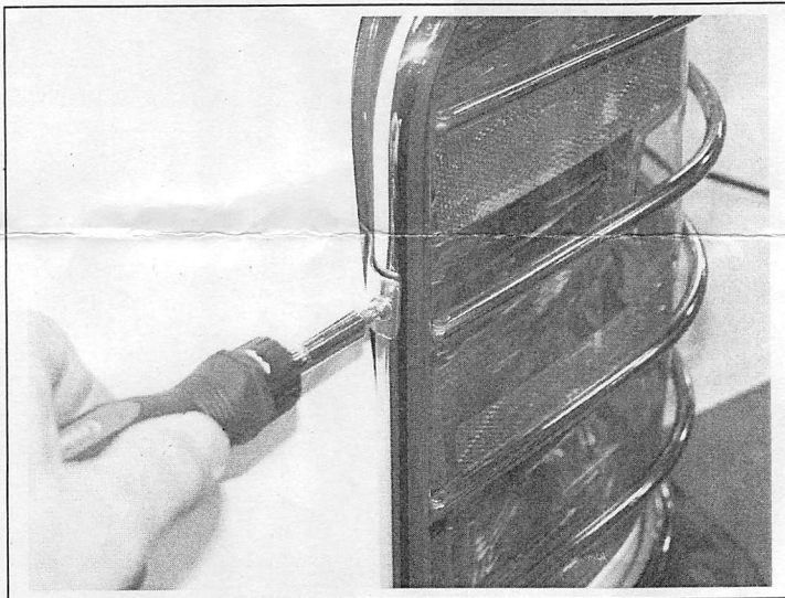
FIG. 4 4mm screw installs through front bracket into threaded insert in guard
