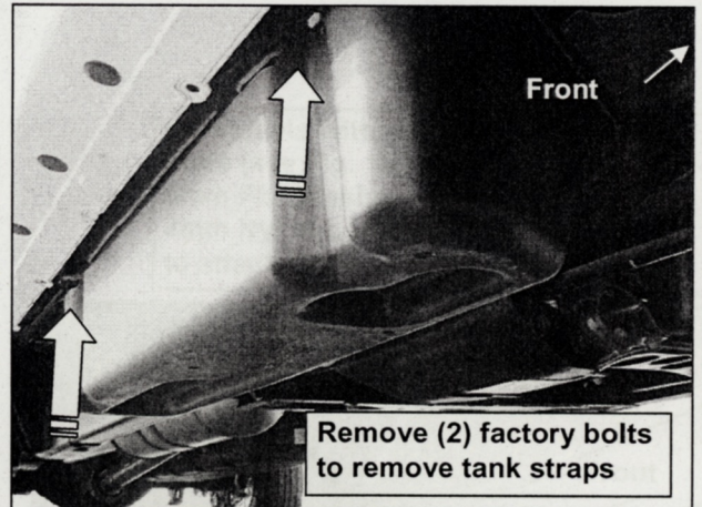
(Fig 12) Passenger side DEF tank and cover Remove (2) factory bolts to remove tank straps
