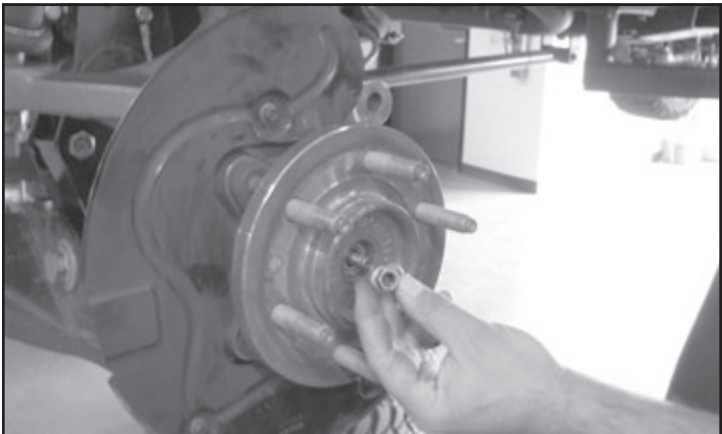
FIGURE 44 - STEP 47
