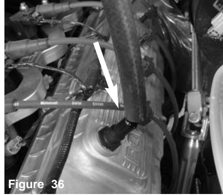
Figure 36 Attach the 15mm hose to the engine fitting.
