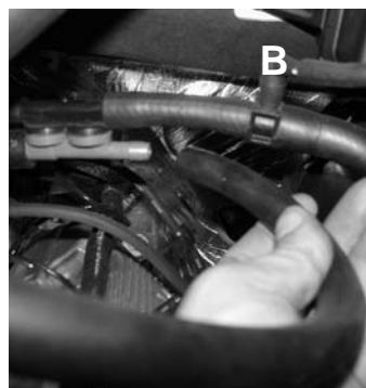
Figure 10 Remove the resonator air box from vehicle.
