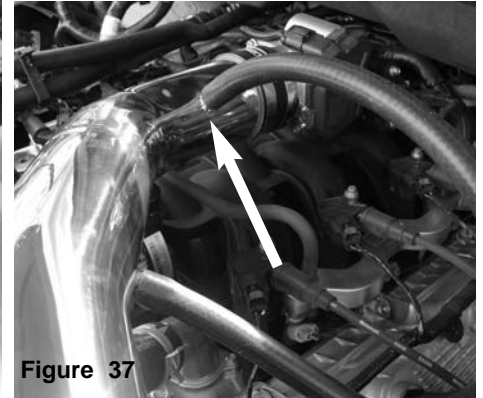
Figure 37 Now install to the fitting on the intake tube closes to the throttle body and secure.
