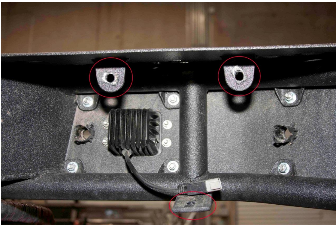
The 3 tabs on the Revolver Rear bumper that will line up with the factory tabs. Re-use the factory hardware to bolt up the rear bumper.
