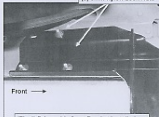
(Fig 4) Driver side front Bracket installation
