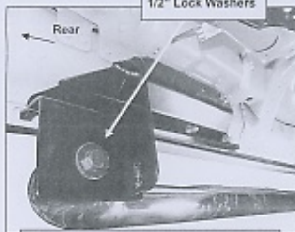
(Fig 6) Driver side rear Bracket installation
