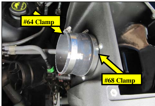
16. Slide the remaining Coupler and Clamps onto the Filter adapter, as shown.
