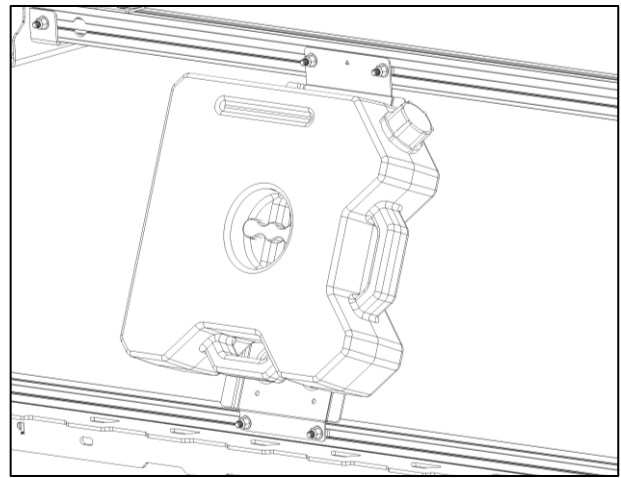
Rotopax mounted horizontally
