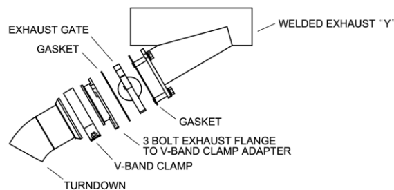
SCHEMATIC 3
