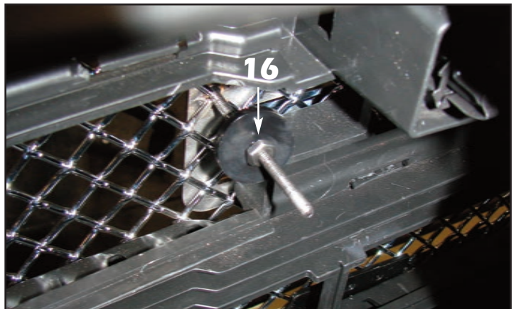
16. Align the black nylon plastic washer over the stud behind the "C" and install a #8-32 ESNA half nut and tighten (mesh grille shown, E-Power mesh grille similar).
