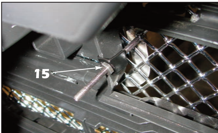
15. Install the emblem mounting bracket over the stud behind the "G" and install a #8-32 ESNA half nut and tighten (mesh grille shown, E-Power mesh grille similar).
