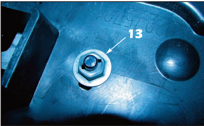
13. Align the factory emblem over the mesh grille, making sure the alignment pins pass through the factory holes in the plastic. Install the supplied speed nuts onto the factory alignment pins on the back of the GMC emblem and once started, turn the nut an additional 1/4 to 1/2 turn to secure.
