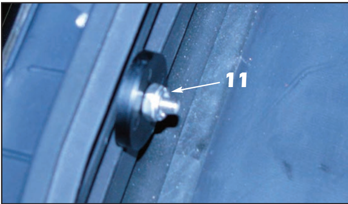
11. Install the supplied large black plastic washers across the bottom of the grille using the supplied #8-32 ESNA half nuts and tighten until the washers no longer freely rotate.
