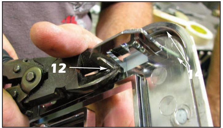
12. For customers requesting emblem reinstallation: Cut the factory mounting tabs from the back of the emblem, making sure you leave the two 3/16" diameter alignment pins in place.
